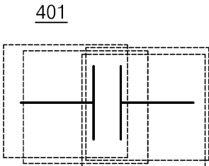
(b)Detected symbols
